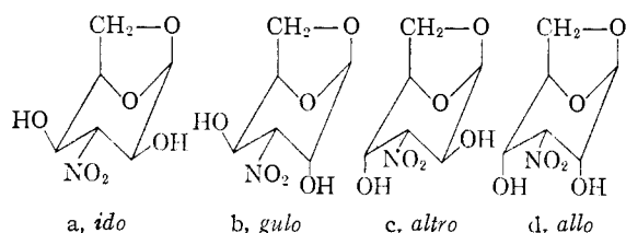
Fig. 1.—Conformations of the four possible isomers in which the nitro group is equatorial.
